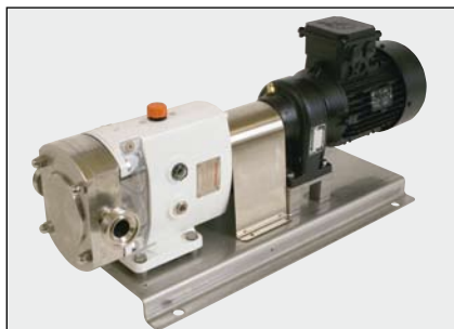
Lobrotorpump 2/013
